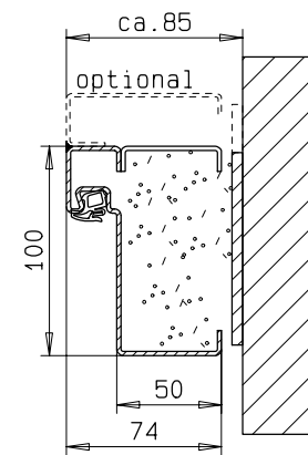
flexible wall
